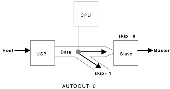
Figure 9-34. Skip or Commit, AUTOOUT=0
