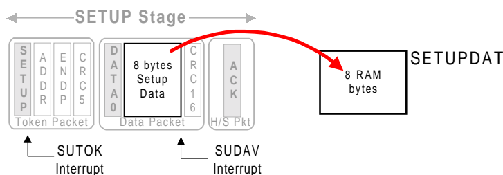
Figure 2-2. Two Interrupts Associated with EPO CONTROL Transfers
