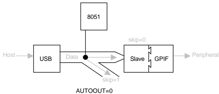
Figure 10-47. Firmware can Skip or Commit, AUTOOUT = 0
