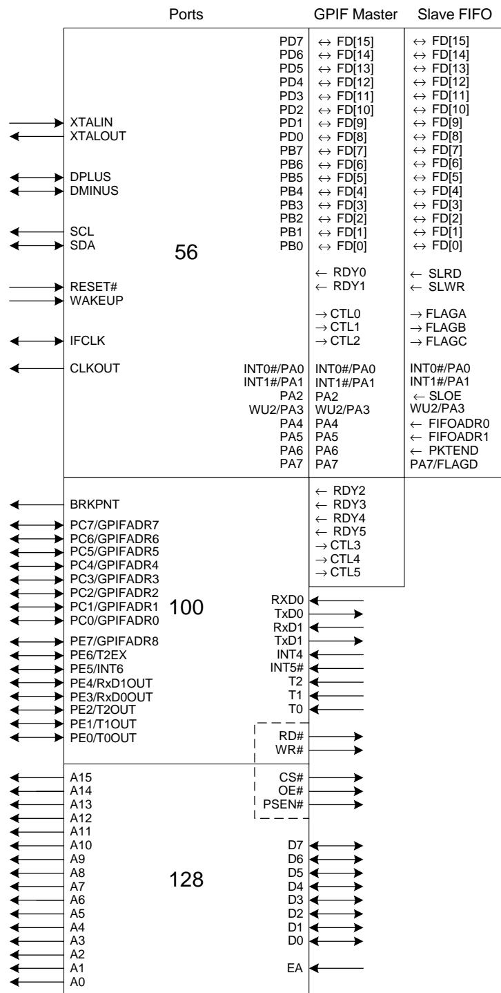
Figure 1-11. Signals for the Three FX2 Package Types
