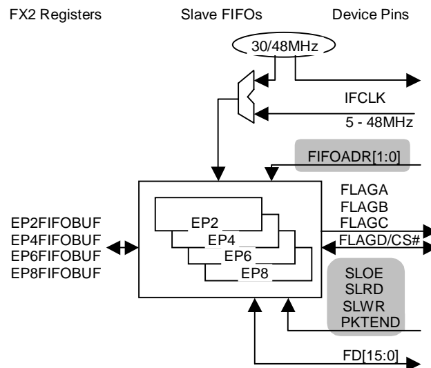
Figure 9-9. Slave FIFO Control Pins
