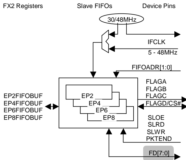
Figure 9-4. 8-bit Mode Slave FIFOs, WORDWIDE=0
