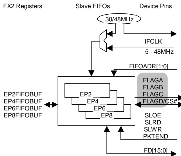
Figure 9-8. FLAGx Role
