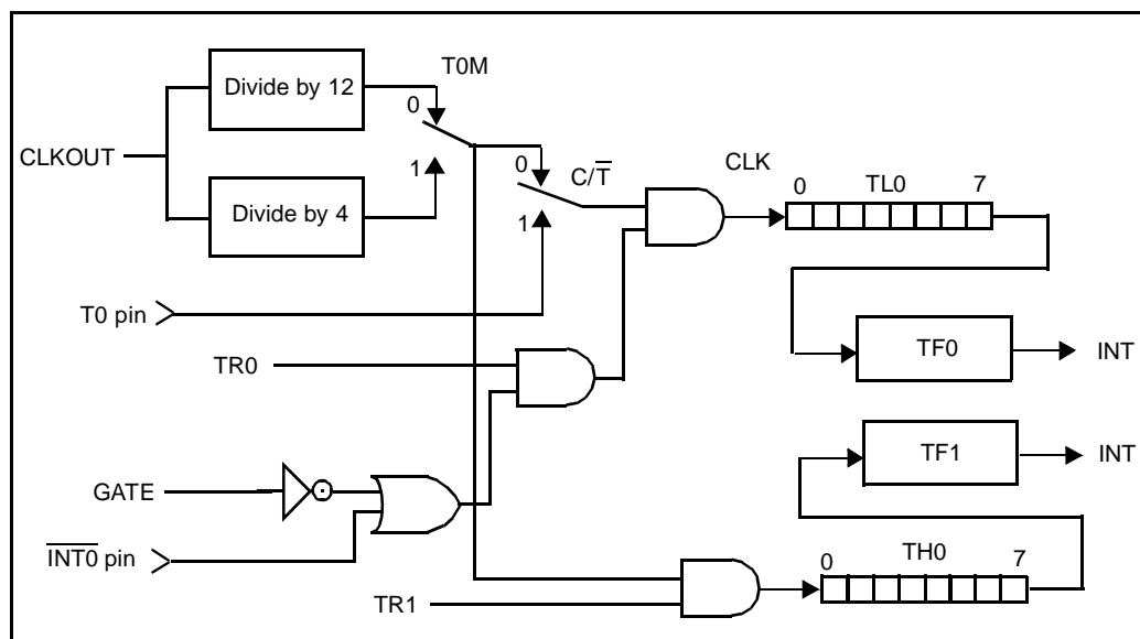
Figure 14-3. Timer 0 - Mode 3
