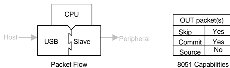
Figure 9-26. Firmware Access to OUT Data
