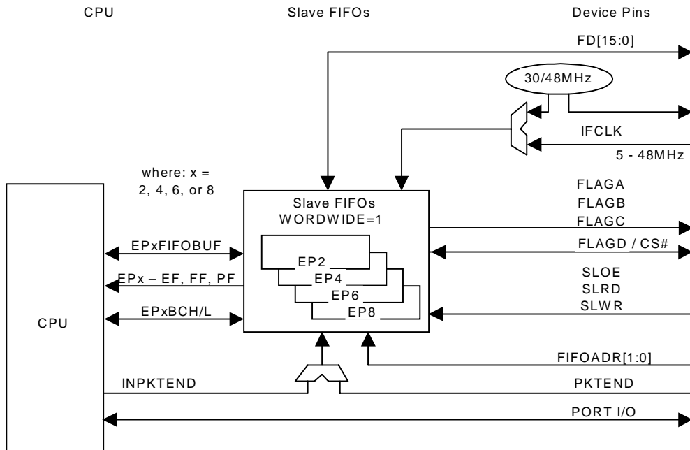
Figure 9-1. Slave FIFOs' Role in the FX2 System
