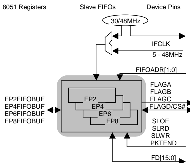
Figure 9-28. EPx Memories
