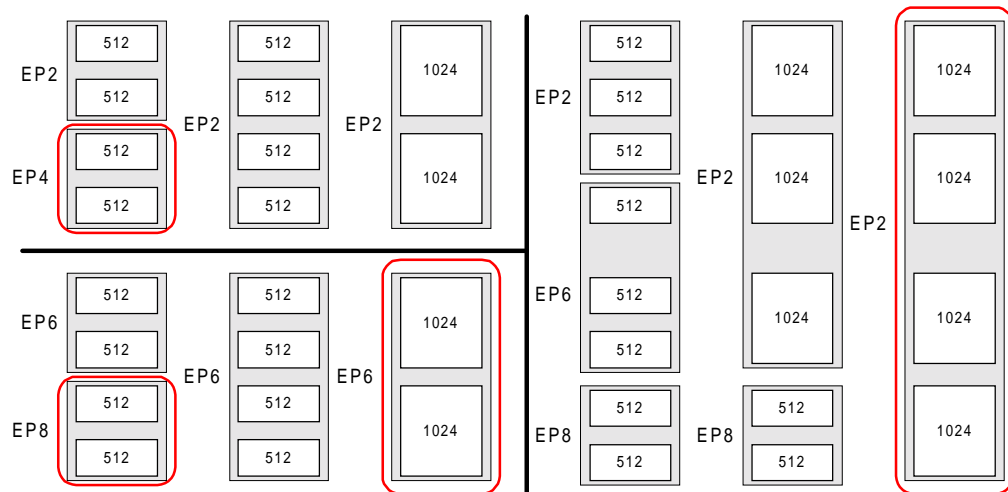
Figure 15-32. Maximum FIFO Sizes
