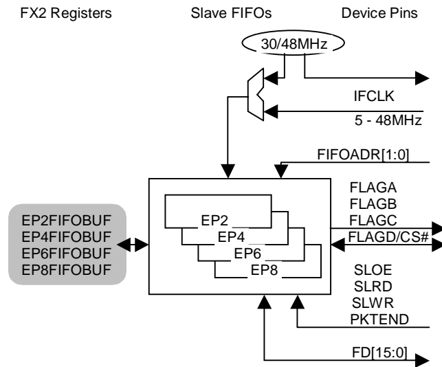
Figure 9-27. EPxFIFOBUF Registers
