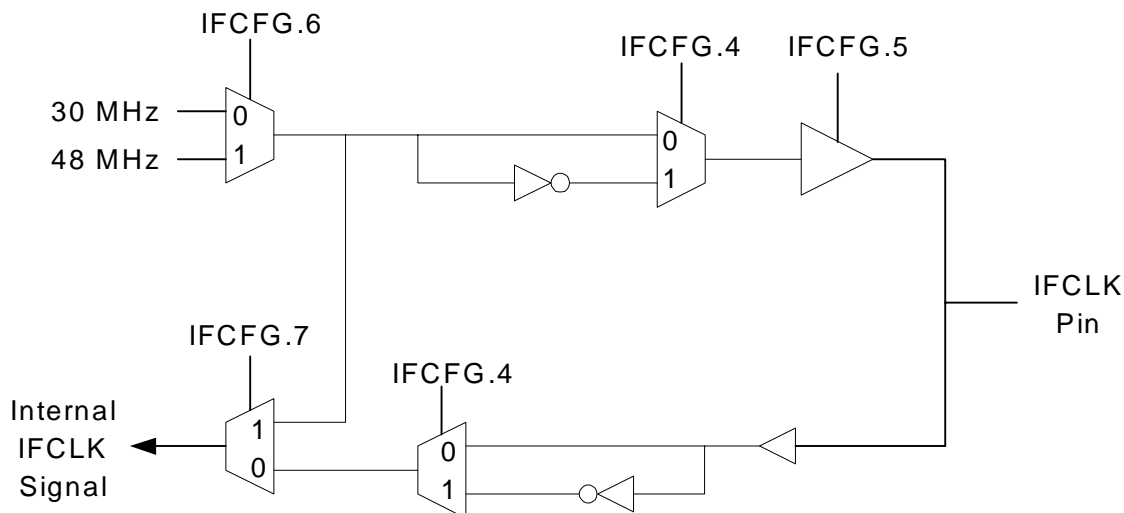
Figure 15-9. IFCLK Configuration
