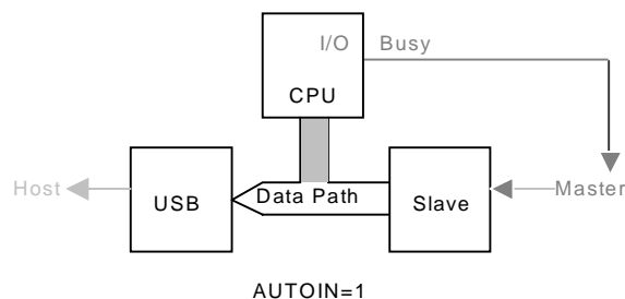
Figure 9-40. Master Writes Directly to Host, AUTOIN = 1
