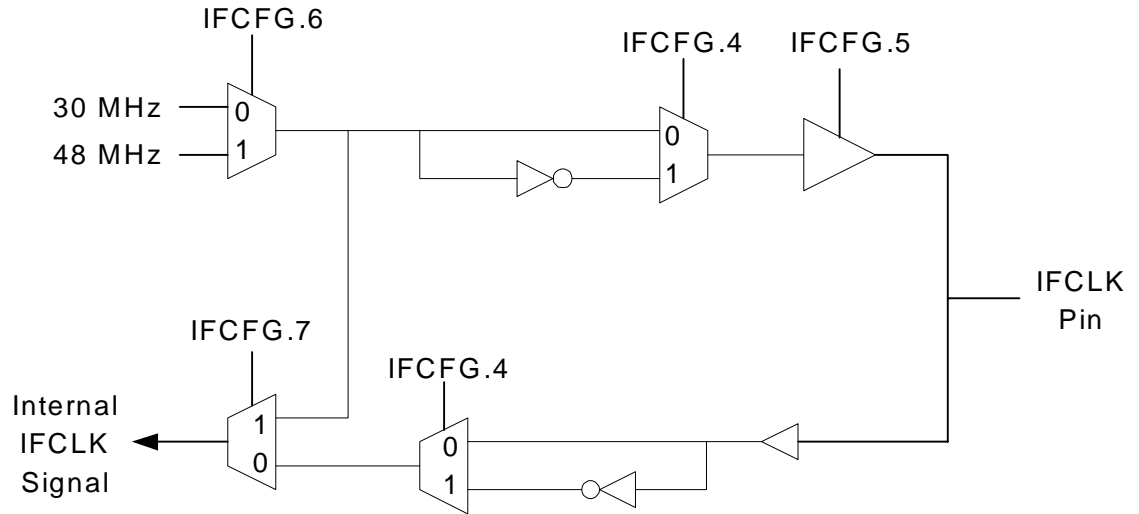
Figure 10-4. IFCLK Configuration
