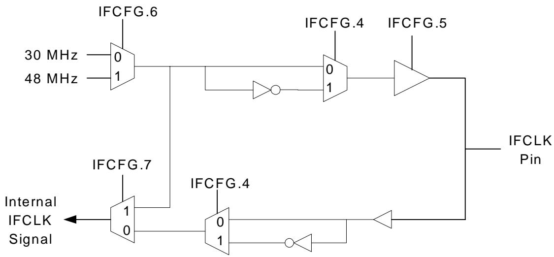
Figure 9-6. IFCLK Configuration
