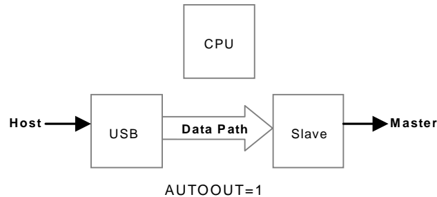
Figure 9-29. When AUTOOUT=1, OUT Packets are Automatically Committed
