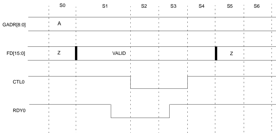
Figure 10-8. One Decision Point: Wait States Inserted Until RDY0 Goes Low
