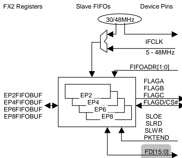
Figure 9-5. 16-bit Mode Slave FIFOs, WORDWIDE=1
